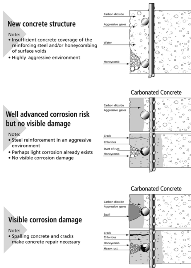
Fig. 2—Concrete with chloride and CO 2 penetration and corrosion.
