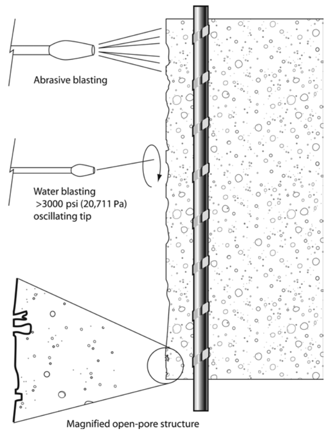
Fig. 3—Surface preparation.
