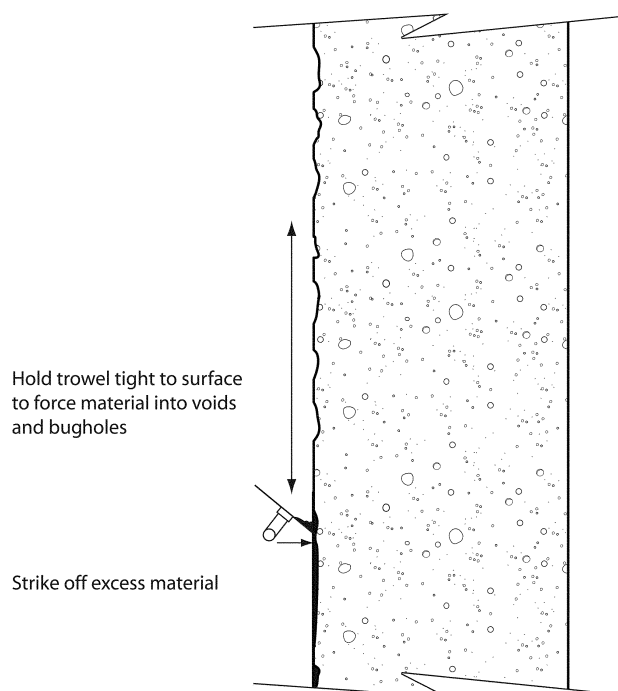
Fig. 4—Troweling material.
