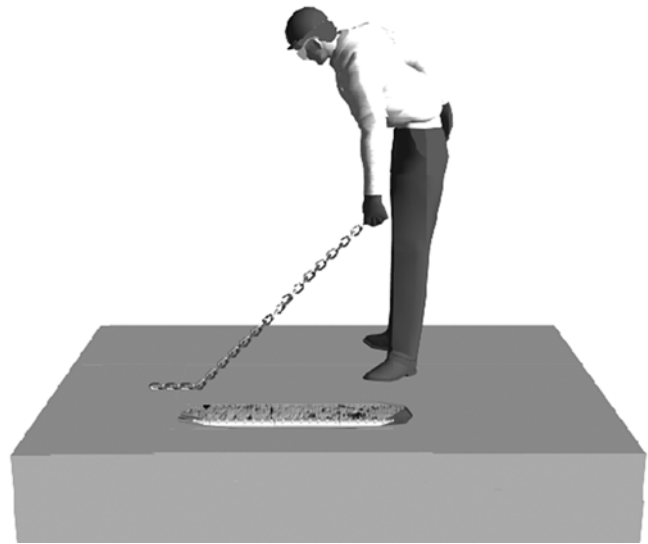
Fig. 1—Sound the concrete surface to locate delaminated areas. Chain drags can be used for sounding.
