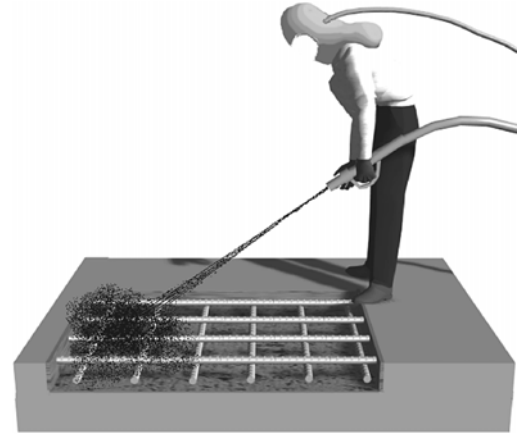
Fig. 7—Clean the exposed concrete and reinforcing bars with high-pressure water or abrasive blasting.
